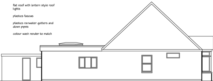
West Elevation
